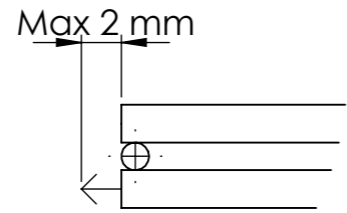
DETAIL D SCALE 2 : 3
